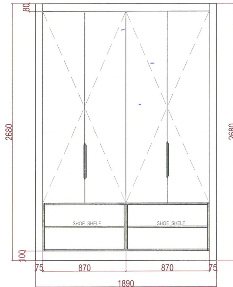
GUEST ROOM WARDROBE- FRONT VIEW
