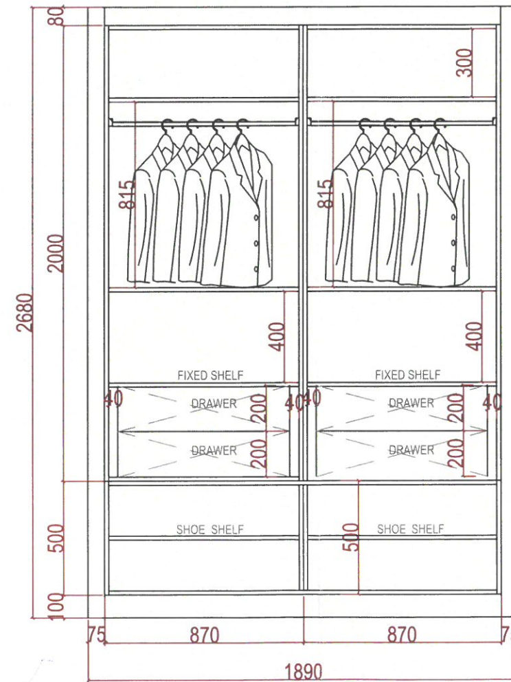
GUEST ROOM WARDROBE- INNER VIEW
