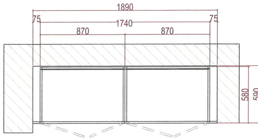
GUEST ROOM WARDROBE- LAYOUT
