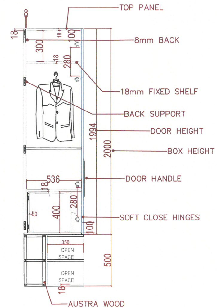
SECTION
